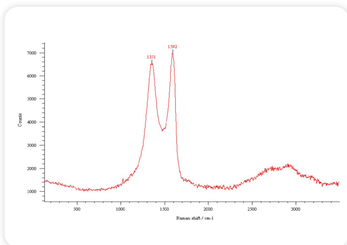
AEROFEN Graphene Oxide RAMAN Results
