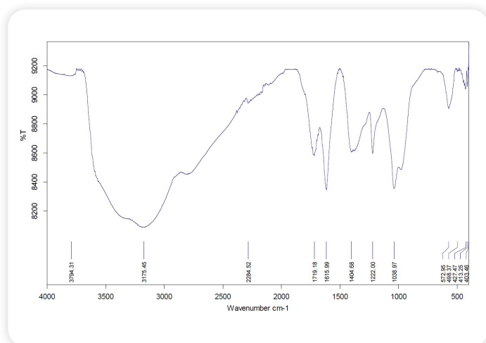
AEROFEN Graphene Oxide FTIR Results
