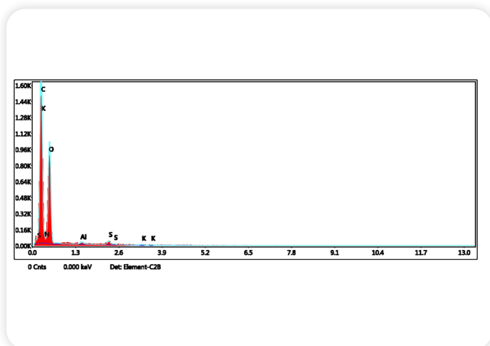
AEROFEN Graphene Oxide EDX Results
