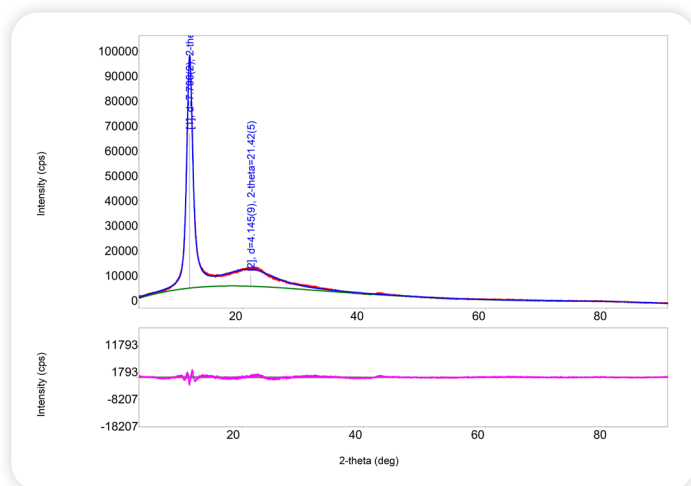
AEROFEN Graphene Oxide XRD Results
